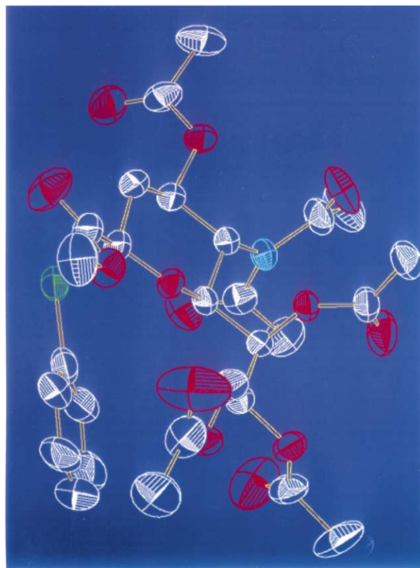
Figure 2. An ORTEP 10 diagram showing the molecular structure of compound 10 . The thermal ellipsoids are drawn with 50% probability. The coloring scheme followed is green (sulfur), red (oxygen), blue (nitrogen), and white (carbon).
