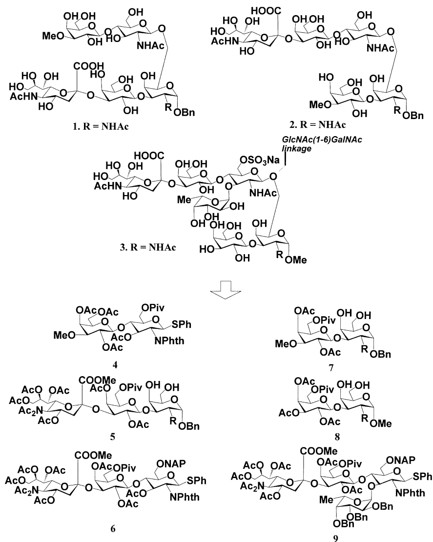
Scheme 1. Target oligosaccharide structures 1–3 and retrosynthetic analyses.
