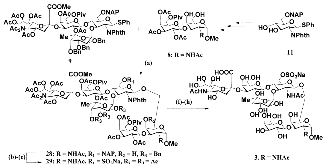
Scheme 6. (a) NIS-TfOH/CH 2 Cl 2 , 4A-MS, -65 to -60 °C, 67%; (b) Ac 2 O-pyridine (1:1), DMAP, rt, 85%; (c) DDQ/CH 2 Cl 2 -CH 3 OH (4:1), rt, 22 h, 75%; (d) SO 3 -pyridine/pyridine, 0–5 °C, 8 h, 85%; (e) Pd/C (10%), H 2 , CH 2 Cl 2 -CH 3 OH, rt, 6 h, then, Ac 2 O-pyridine (1:1), DMAP, rt, 12 h; (f) Lil/pyridine, 120–125 °C, 8 h, N 2 ; (g) CH 3 OH-NH 2 NH 2 -H 2 O, 80–85 °C, 6 h, then Ac 2 O-pyridine (1:1), DMAP, rt, 12 h; (h) 1 M CH 3 ONa-CH 3 OH/CH 3 OH-H 2 O, rt, 12 h, 37% in three steps.
