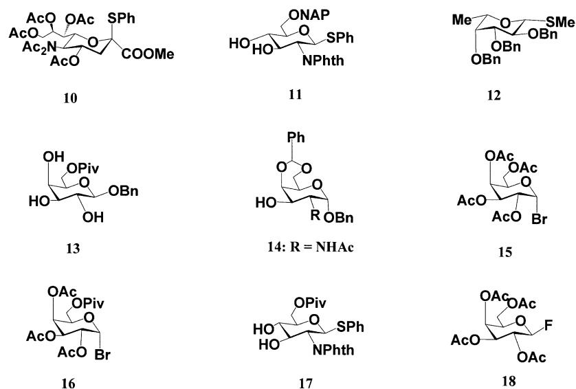
Scheme 2. The intermediate monosaccharide building blocks for target oligosaccharides 1–3.
