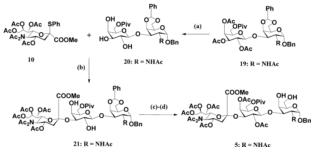
Scheme 3. (a) 1 M CH_3ONa-CH_3OH/CH_2Cl_2-CH_3OH (1:1), -20 to -15^\circ C , 20 min, 85%; (b) NIS-TfOH/ CH_3CN-CH_2Cl_2 (1:1), 3A-MS, -45 to -40^\circ C , 16 h, 45%; (c) Ac_2O -pyridine (1:1), DMAP, rt, 12 h; (d) 60% HOAc, 65^\circ C , 1.5 h, 72% in two steps.
