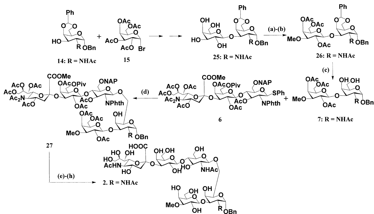
Scheme 5. (a) (i) \text{Bu}_3\text{SnO} /benzene, reflux, 4 h; (ii) \text{CH}_3\text{I} - \text{Bu}_4\text{NI} /benzene-DMF, 40–50 °C, 4 days, 65%; (b) \text{Ac}_2\text{O} -pyridine (1:1), DMAP, rt, 12 h, 85%; (c) 60% \text{HOAc} , 65 °C, 1 h; (d) \text{NIS} - \text{TfOH} / \text{CH}_2\text{Cl}_2 , 4A-MS, –65 to –60 °C, 49%; (e) \text{DDQ} / \text{CH}_2\text{Cl}_2 - \text{CH}_3\text{OH} (4:1), rt, 20 h, 70%; (f) \text{LiI} /pyridine, 120–125 °C, 8 h, \text{N}_2 ; (g) \text{CH}_3\text{OH} - \text{NH}_2\text{NH}_2 - \text{H}_2\text{O} , 80–85 °C, 6 h, then \text{Ac}_2\text{O} -pyridine (1:1), DMAP, rt, 12 h; (h) 1 M \text{CH}_3\text{ONa} - \text{CH}_3\text{OH} / \text{CH}_3\text{OH} - \text{H}_2\text{O} , rt, 12 h, 33% in three steps.
