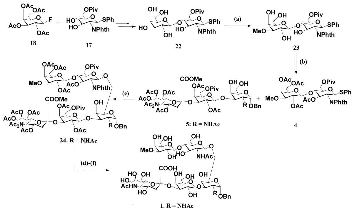
Scheme 4. (a) (i) Bu_3SnO /benzene, reflux, 4 h; (ii) CH_3I-Bu_4NI /benzene-DMF, 40-50^\circ C , 4 days, 68%; (b) Ac_2O -pyridine (1:1), DMAP, rt, 12 h, 90%; (c) NIS-TfOH/ CH_2Cl_2 , 4A-MS, -65 to -60^\circ C , 65%; (d) LiI/pyridine, 120-125^\circ C , 8 h, N_2 ; (e) CH_3OH-NH_2NH_2 \cdot H_2O , 80-85^\circ C , 6 h, then Ac_2O -pyridine (1:1), DMAP, rt, 12 h; (f) 1 M CH_3ONa-CH_3OH/CH_3OH-H_2O , rt, 12 h, 37% in three steps.
