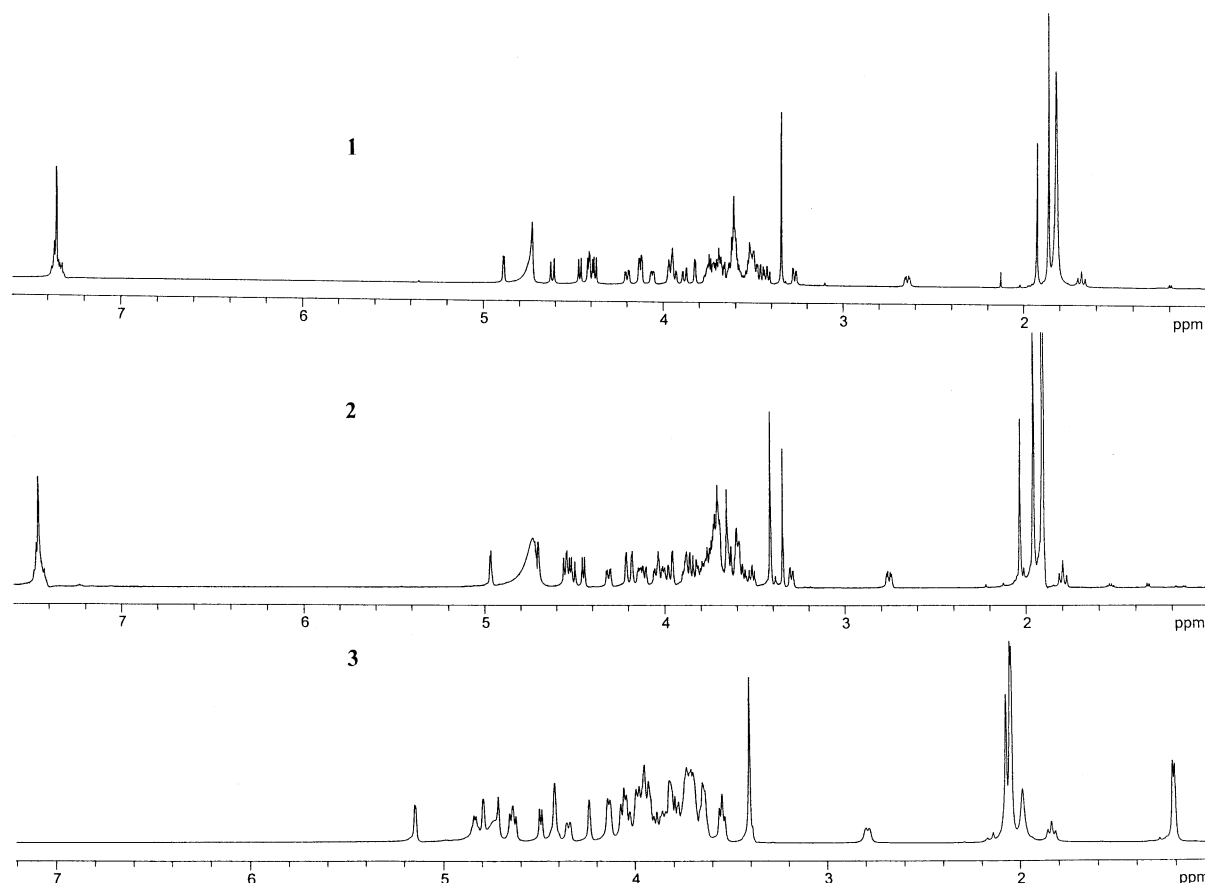
Figure 3. 600 MHz 1D 1 H NMR of oligosaccharides: 1 (D 2 O), 2 (D 2 O + CD 3 OD) and 3 (D 2 O) recorded at 303.0 K.
